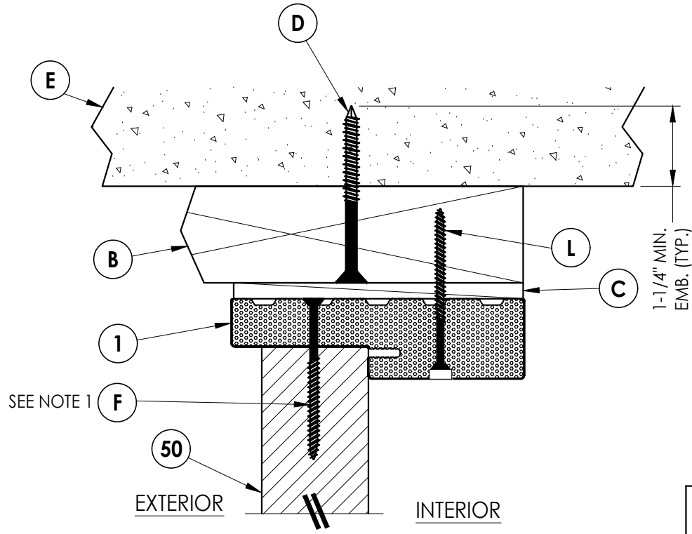
3 4 VERTICAL CROSS SECTION Shown with 2X Buck Outswing
