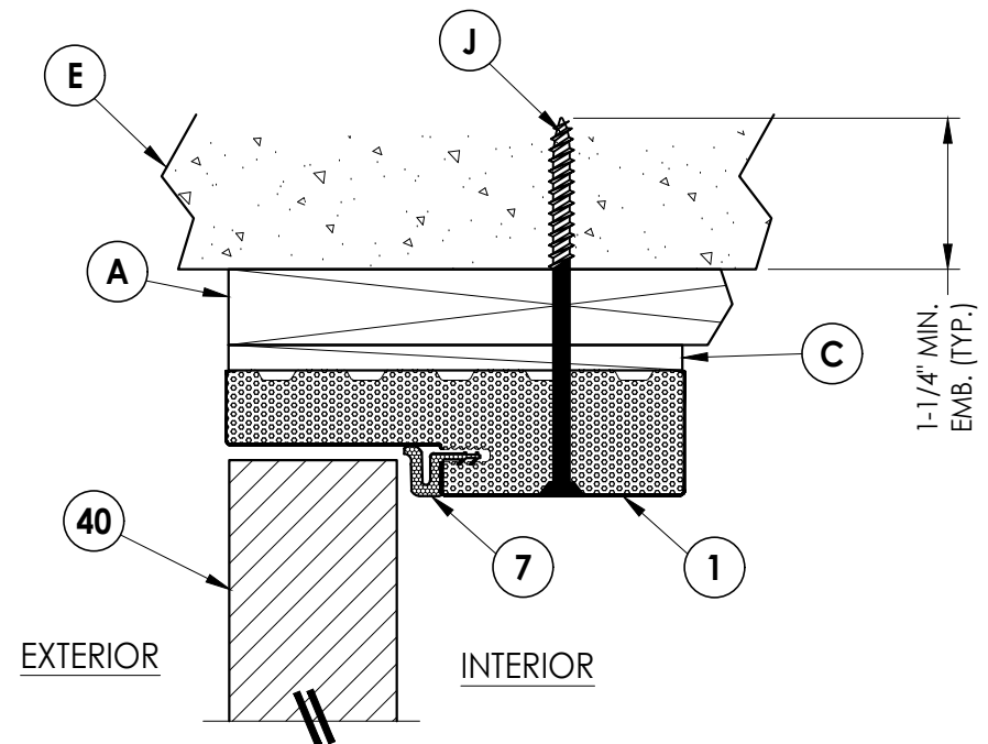
2 4 VERTICAL CROSS SECTION Shown with 1X Buck Outswing
