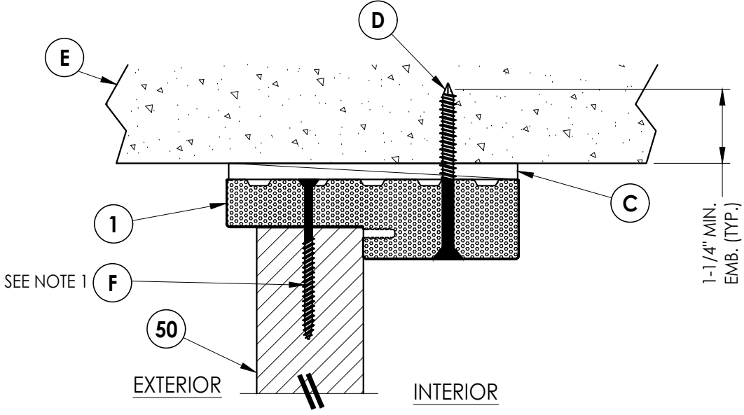
4 4 VERTICAL CROSS SECTION Shown Direct to Masonry Outswing
