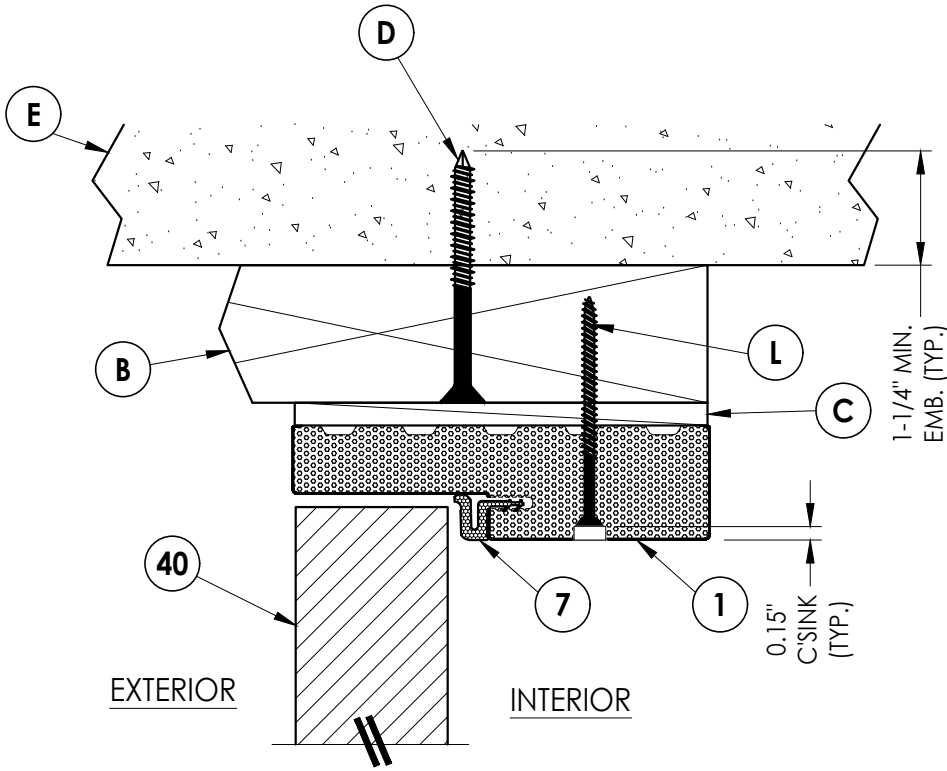
1 4 VERTICAL CROSS SECTION Shown with 2X Buck Outswing
